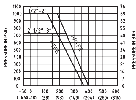
Pressure Vs Temperature Chart
